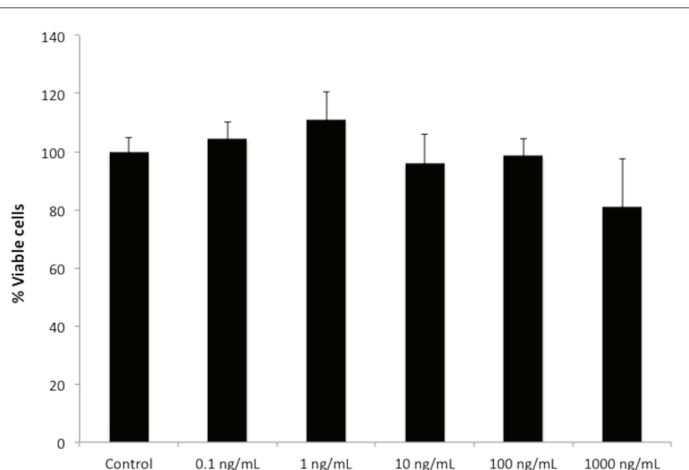
Figure 1: Effects of CdTe-COOH on cell viability of HeLa cells. Cells were exposed in culture medium using different concentrations of CdTe-COOH QDs for 24 h. Results are expressed as the percentage of cell viability as compared to the control group. Data are presented as the mean \pm SD of at least three independent experiments (n=8). *p < 0.05 as compared with control group.
