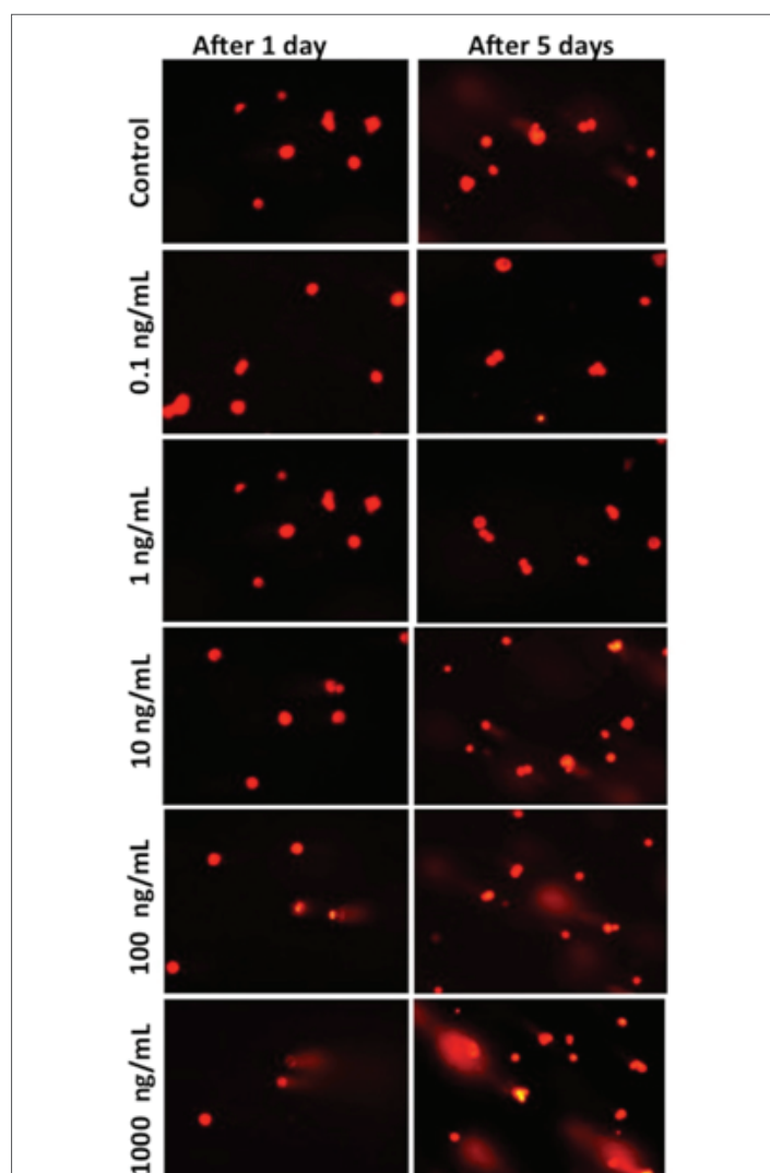
Figure 5: Analysis of \beta -HCP genotoxicity. HeLa cells were treated with CdTe-COOH at 0.1, 1, 10, 100 and 1000 ng/mL for 1 or 5 days. H_2O_2 300 \mu M was used as positive control (control +). Results are expressed as average percentage of tail DNA \pm d.s. Data are presented as the mean \pm SD of at least three independent experiments ( n = 6 ). * p < 0.05 as compared with control group.
