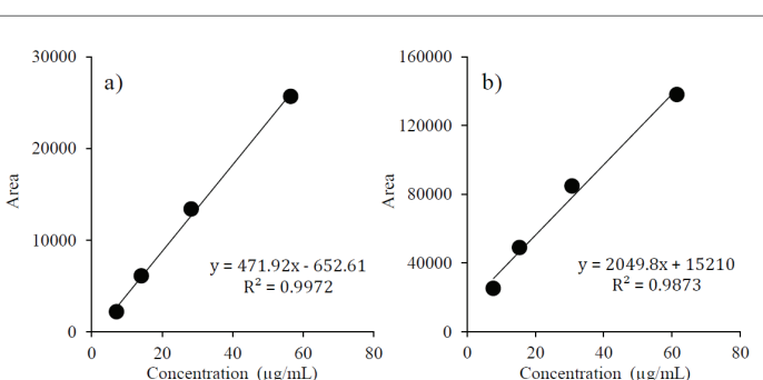
Figure 4: Calibration curves
